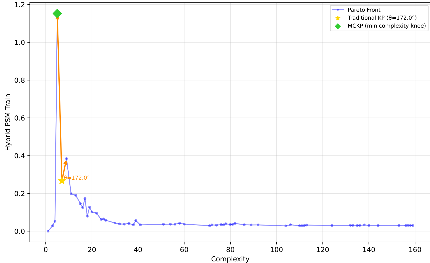
227_cpu_small - Run 24 - SVP - Hybrid PSM Train \lambda_1=0.00, \lambda_2=1.00, \lambda_3=0.00 | Difficulty: 1.00 | Method: hmr
