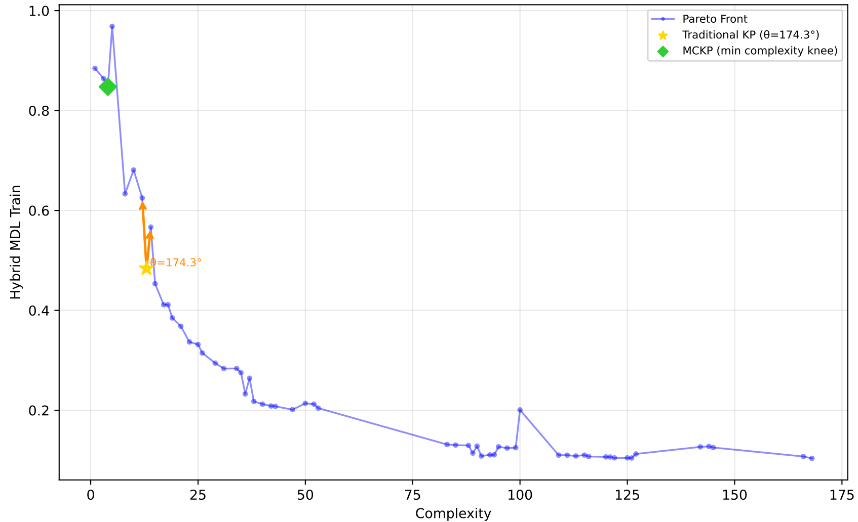
227_cpu_small - Run 25 - MVP - Hybrid MDL Train \lambda_1=0.00, \lambda_2=0.90, \lambda_3=0.10 | Difficulty: 1.00 | Method: hmr
