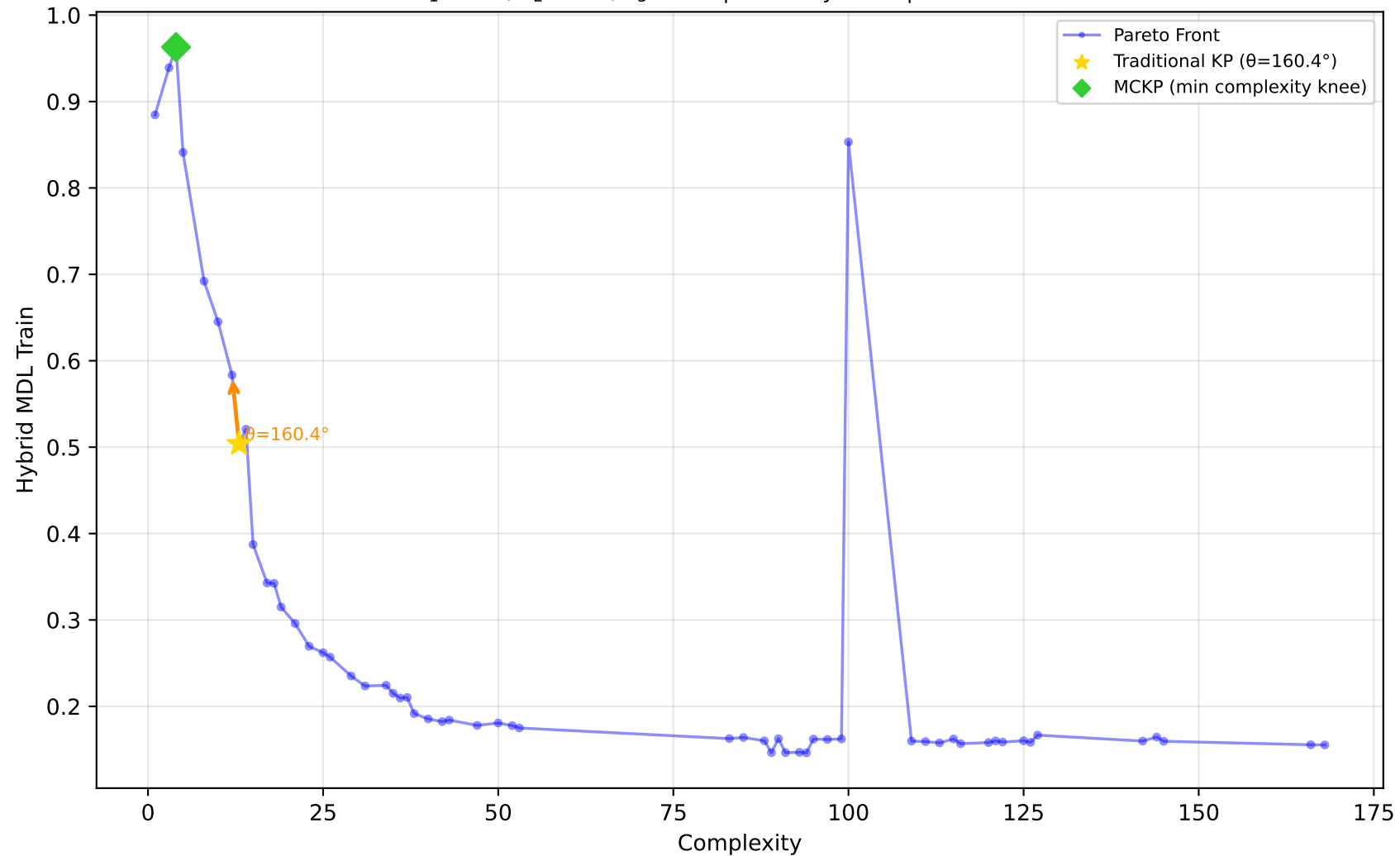
227_cpu_small - Run 25 - MVP - Hybrid MDL Train \lambda_1=0.80, \lambda_2=0.20, \lambda_3=0.00 | Difficulty: 1.00 | Method: hmr
