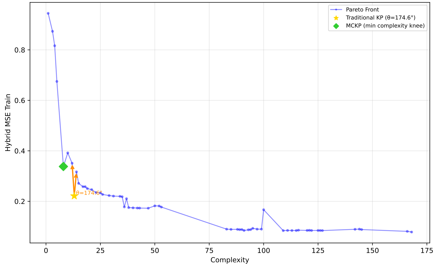
227_cpu_small - Run 25 - MVP - Hybrid MSE Train \lambda_1=0.00, \lambda_2=0.90, \lambda_3=0.10 | Difficulty: 1.00 | Method: hmr
