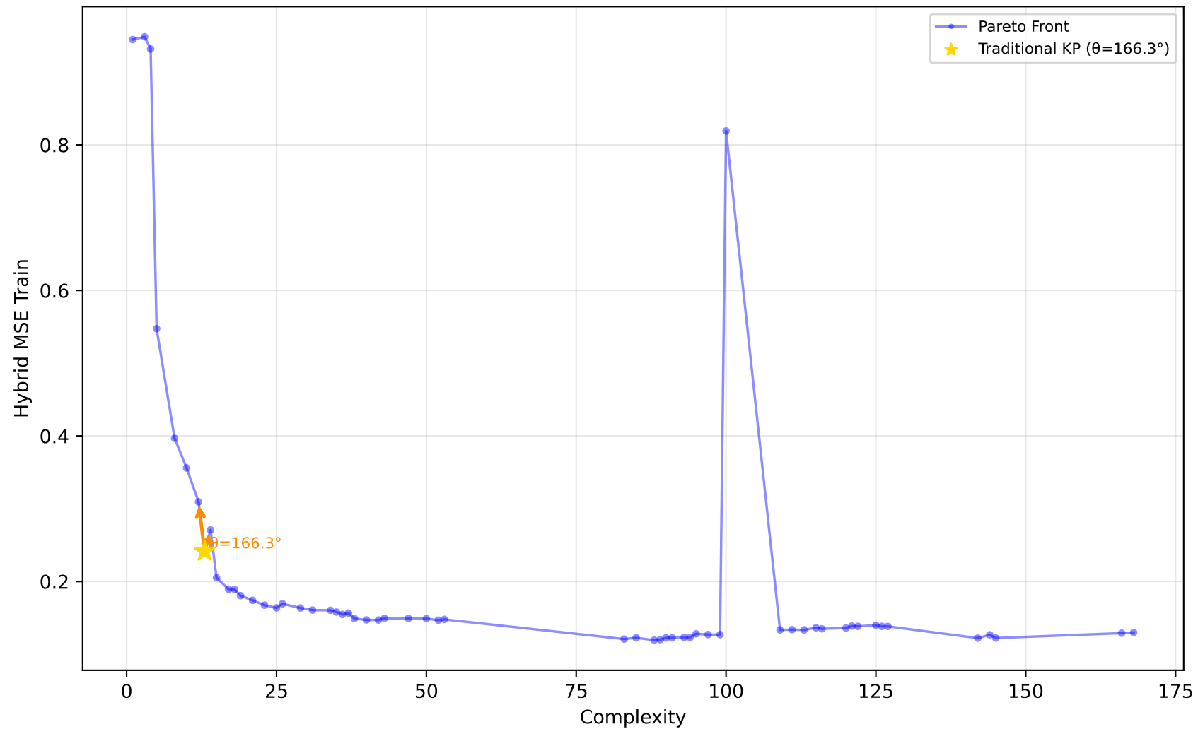
227_cpu_small - Run 25 - MVP - Hybrid MSE Train \lambda_1=0.80, \lambda_2=0.20, \lambda_3=0.00 | Difficulty: 1.00 | Method: hmr
