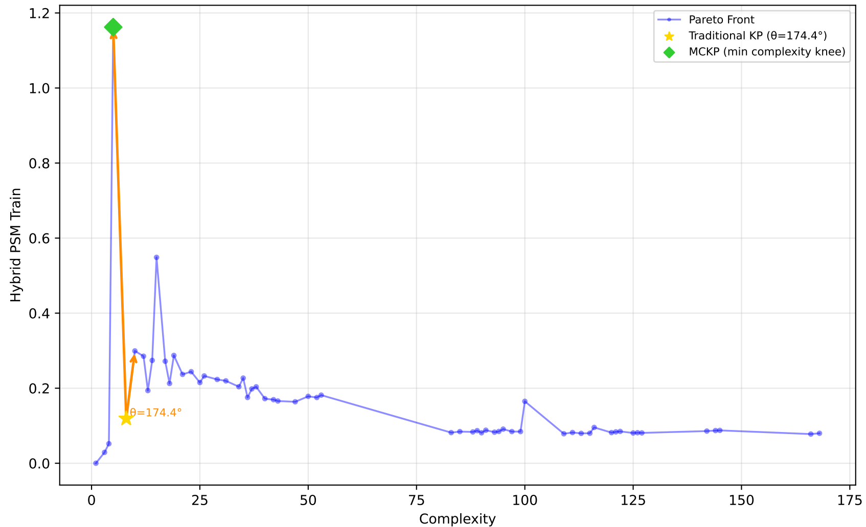
227_cpu_small - Run 25 - MVP - Hybrid PSM Train \lambda_1=0.00, \lambda_2=0.90, \lambda_3=0.10 | Difficulty: 1.00 | Method: hmr
