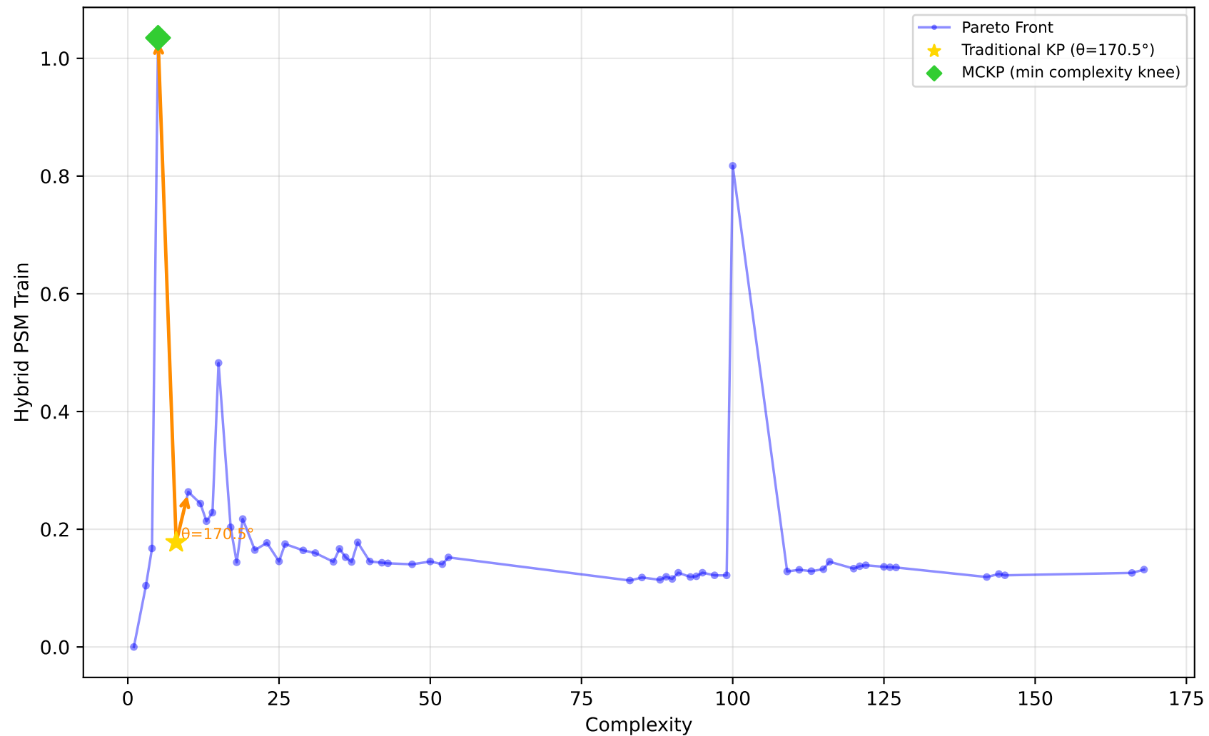
227_cpu_small - Run 25 - MVP - Hybrid PSM Train \lambda_1=0.80, \lambda_2=0.20, \lambda_3=0.00 | Difficulty: 1.00 | Method: hmr
