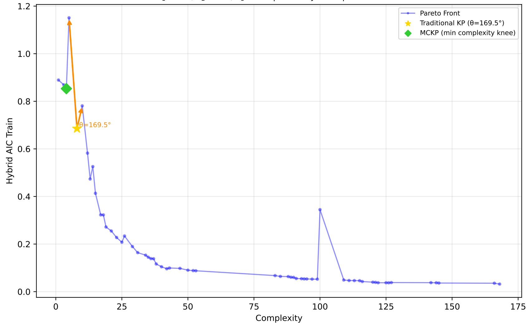
227_cpu_small - Run 25 - SVP - Hybrid AIC Train \lambda_1=0.00, \bar{\lambda}_2=0.80, \lambda_3=0.30 | Difficulty: 1.00 | Method: hmr
