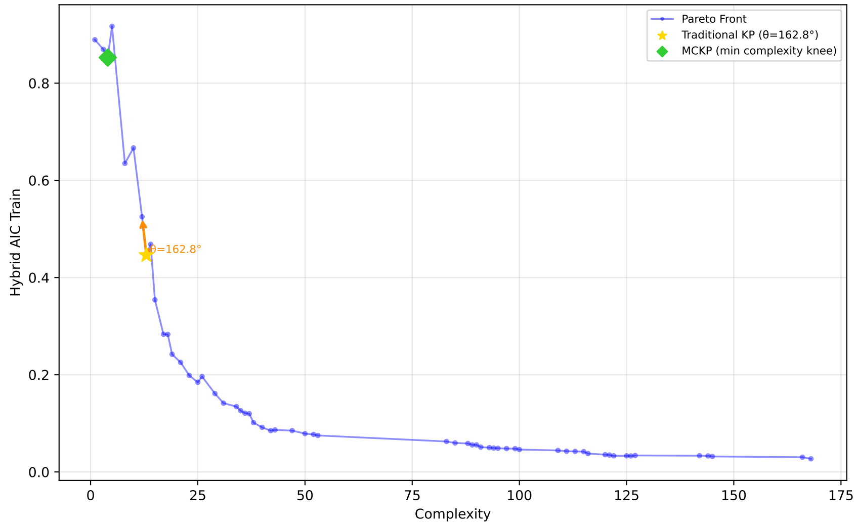
227_cpu_small - Run 25 - SVP - Hybrid AIC Train \lambda_1=0.00, \bar{\lambda}_2=1.00, \lambda_3=0.00 | Difficulty: 1.00 | Method: hmr
