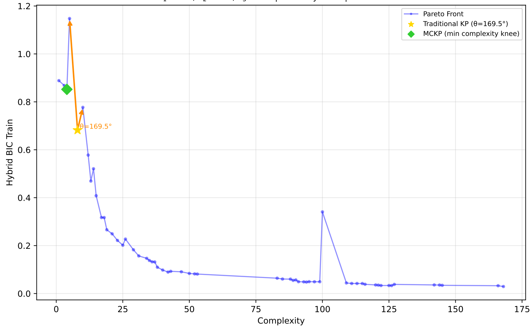
227_cpu_small - Run 25 - SVP - Hybrid BIC Train \lambda_1=0.00, \bar{\lambda}_2=0.80, \lambda_3=0.30 | Difficulty: 1.00 | Method: hmr
