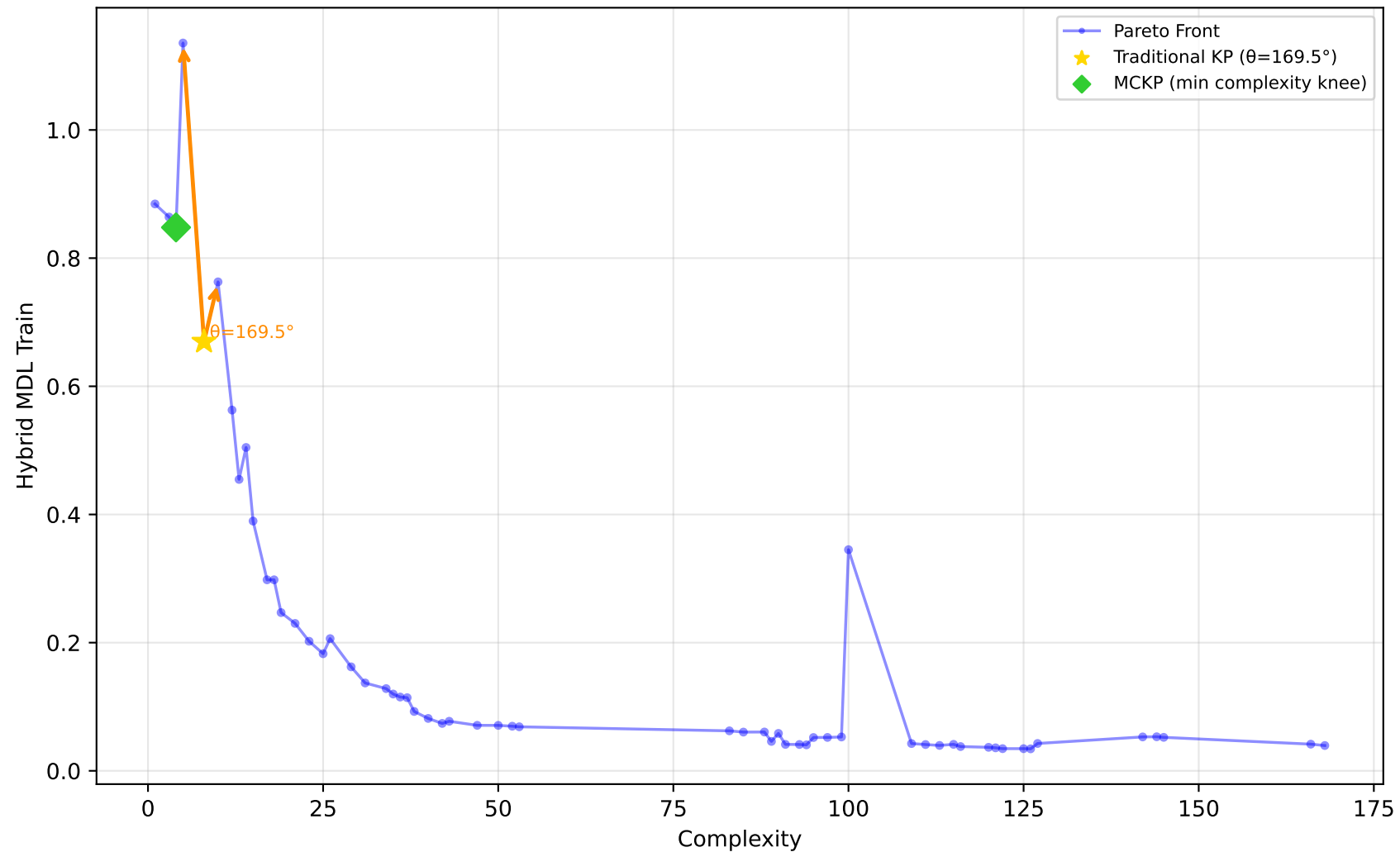
227_cpu_small - Run 25 - SVP - Hybrid MDL Train \lambda_1=0.00, \lambda_2=0.80, \lambda_3=0.30 | Difficulty: 1.00 | Method: hmr
