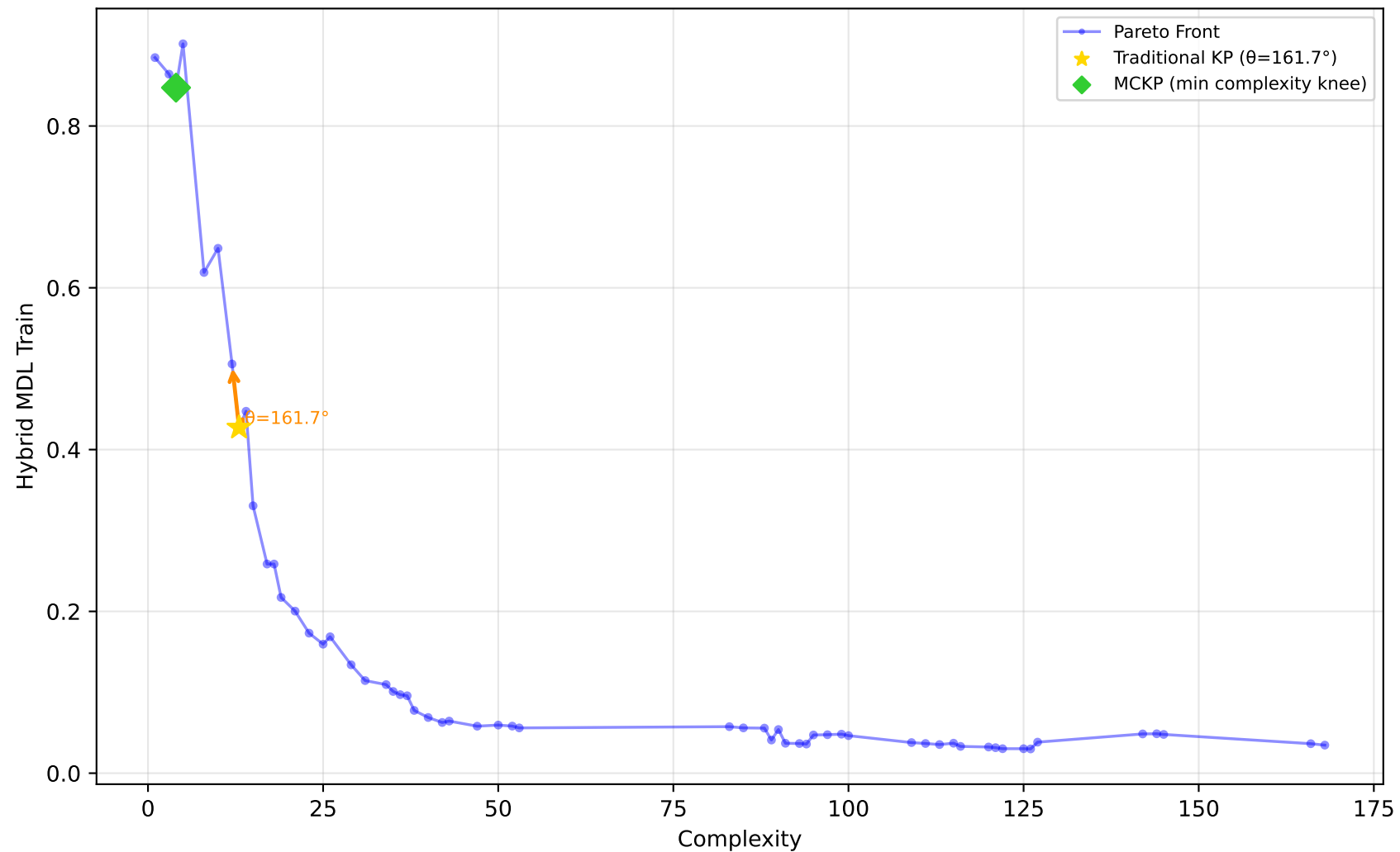
227_cpu_small - Run 25 - SVP - Hybrid MDL Train \lambda_1=0.00, \lambda_2=1.00, \lambda_3=0.00 | Difficulty: 1.00 | Method: hmr
