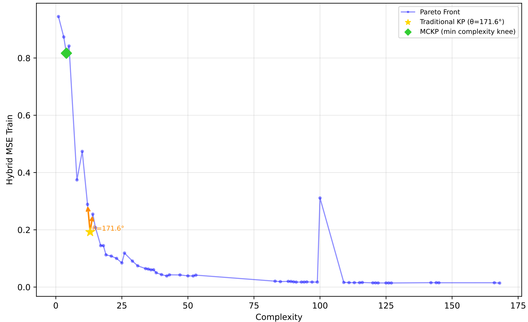
227_cpu_small - Run 25 - SVP - Hybrid MSE Train \lambda_1=0.00, \lambda_2=0.80, \lambda_3=0.30 | Difficulty: 1.00 | Method: hmr
