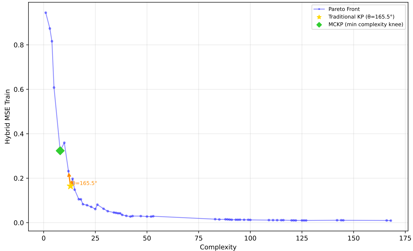
227_cpu_small - Run 25 - SVP - Hybrid MSE Train \lambda_1=0.00, \lambda_2=1.00, \lambda_3=0.00 | Difficulty: 1.00 | Method: hmr
