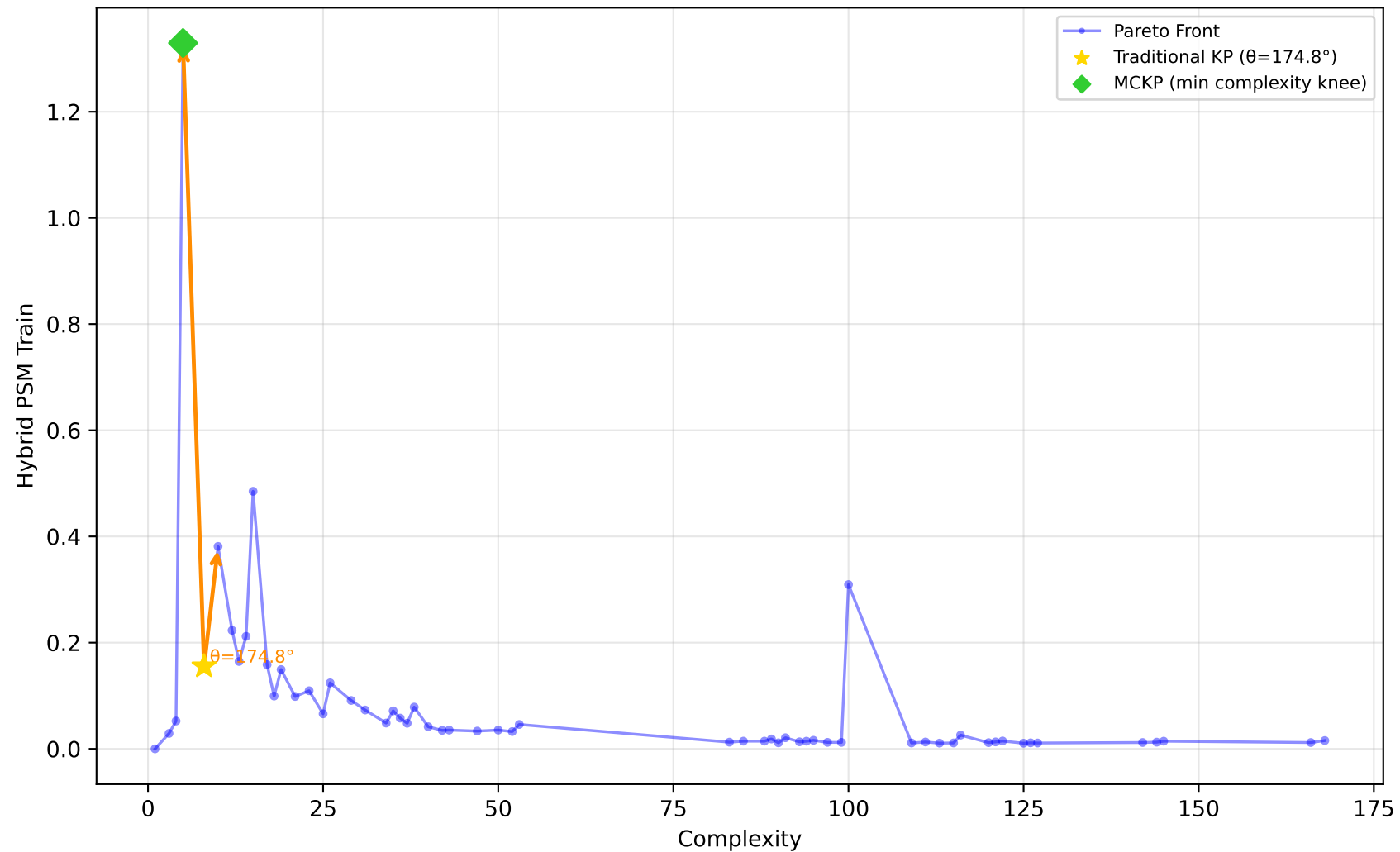
227_cpu_small - Run 25 - SVP - Hybrid PSM Train \lambda_1=0.00, \lambda_2=0.80, \lambda_3=0.30 | Difficulty: 1.00 | Method: hmr
