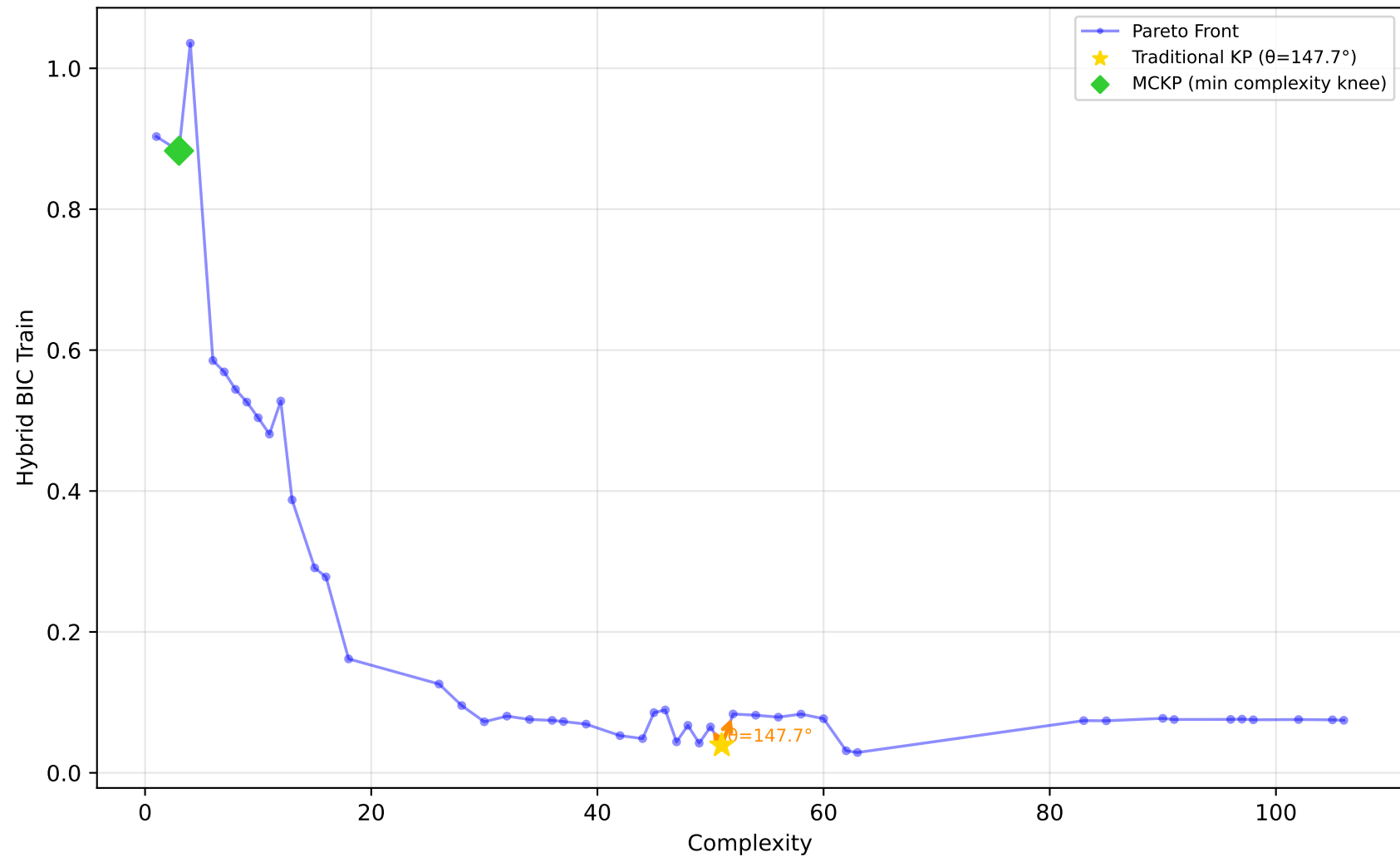
227_cpu_small - Run 26 - MVP - Hybrid BIC Train \lambda_1=0.00, \lambda_2=0.90, \lambda_3=0.10 | Difficulty: 1.00 | Method: hmr
