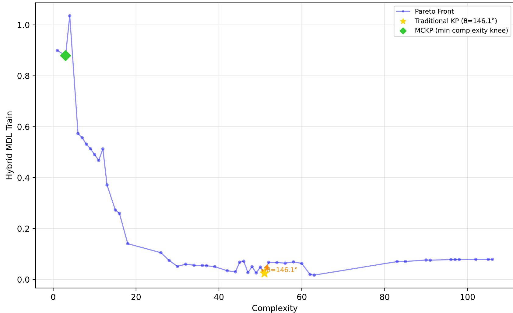
227_cpu_small - Run 26 - MVP - Hybrid MDL Train \lambda_1=0.00, \lambda_2=0.90, \lambda_3=0.10 | Difficulty: 1.00 | Method: hmr
