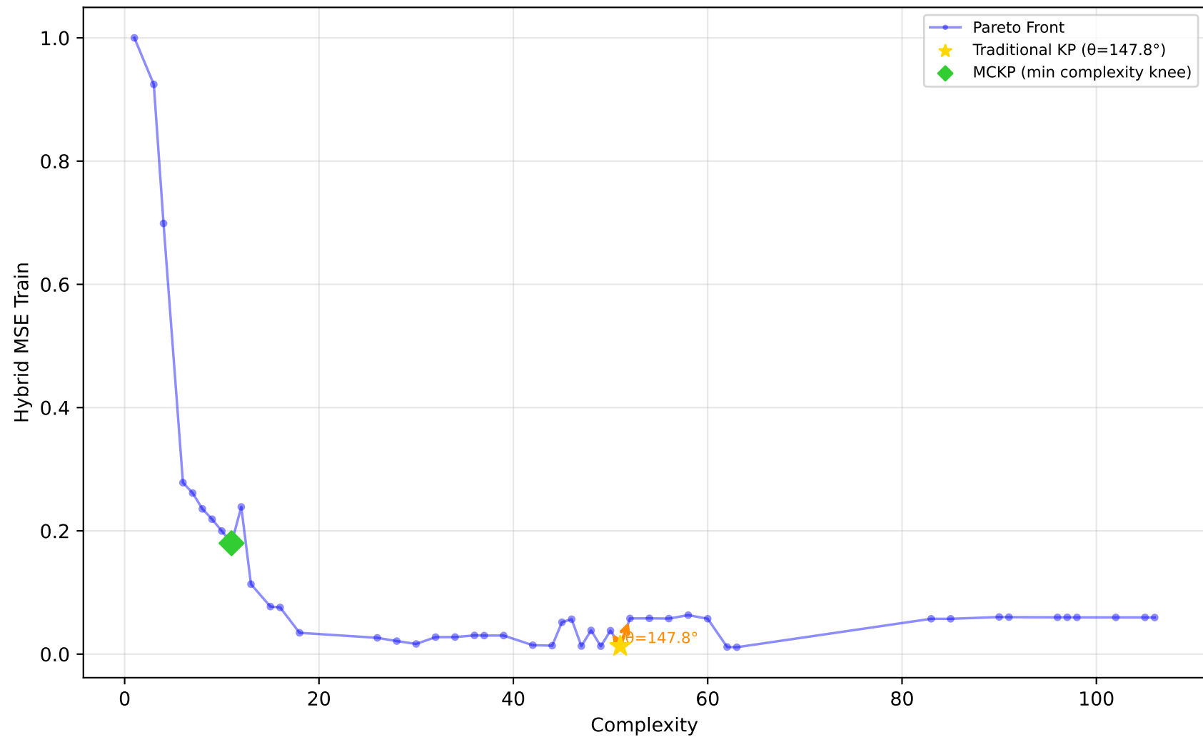
227_cpu_small - Run 26 - MVP - Hybrid MSE Train \lambda_1=0.00, \lambda_2=0.90, \lambda_3=0.10 | Difficulty: 1.00 | Method: hmr
