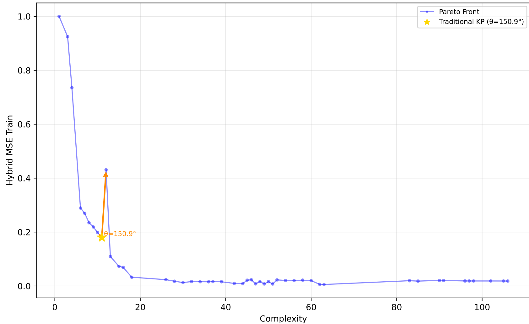
227_cpu_small - Run 26 - SVP - Hybrid MSE Train \lambda_1=0.00, \lambda_2=0.80, \lambda_3=0.30 | Difficulty: 1.00 | Method: hmr
