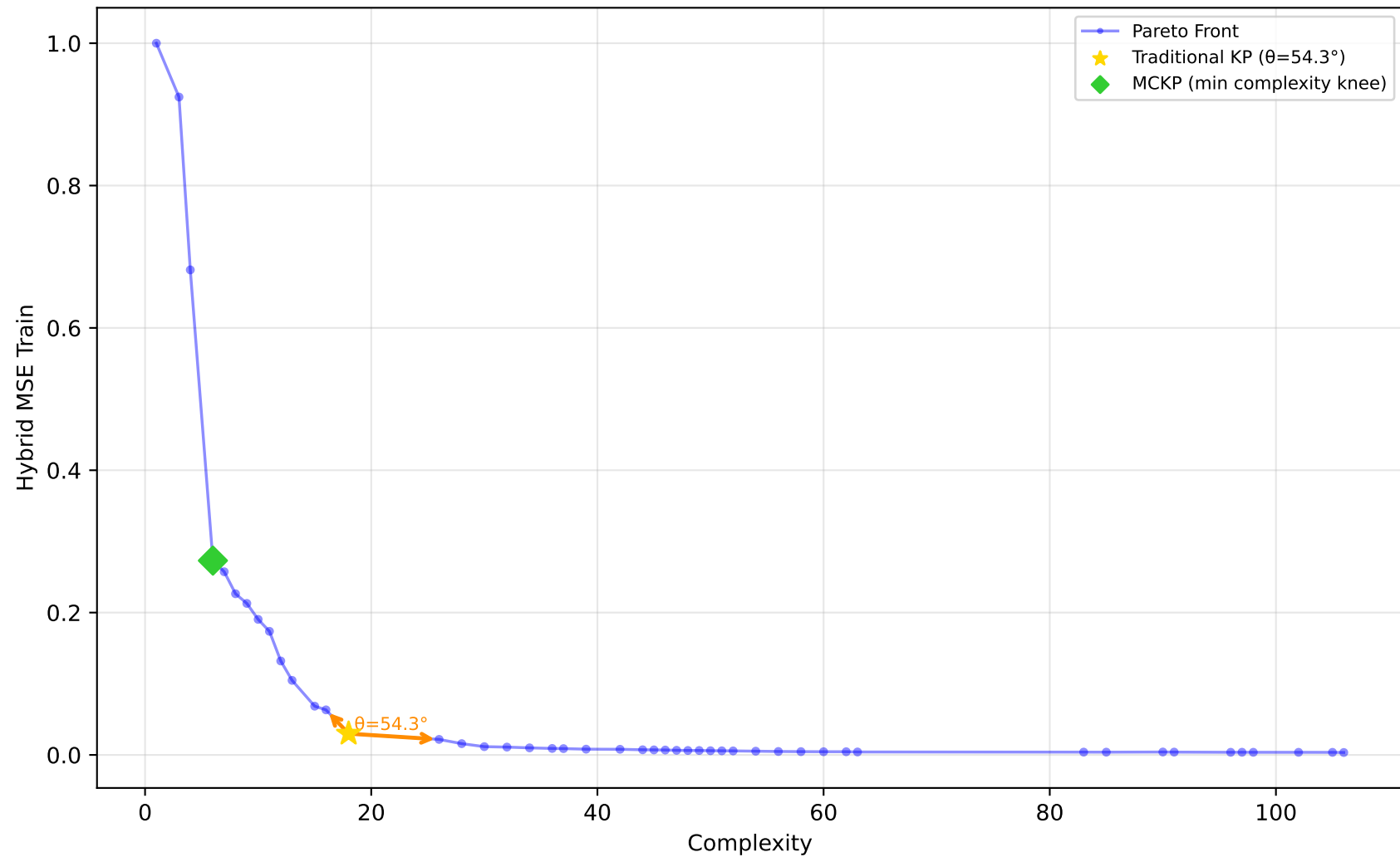
227_cpu_small - Run 26 - SVP - Hybrid MSE Train \lambda_1=0.00, \lambda_2=1.00, \lambda_3=0.00 | Difficulty: 1.00 | Method: hmr
