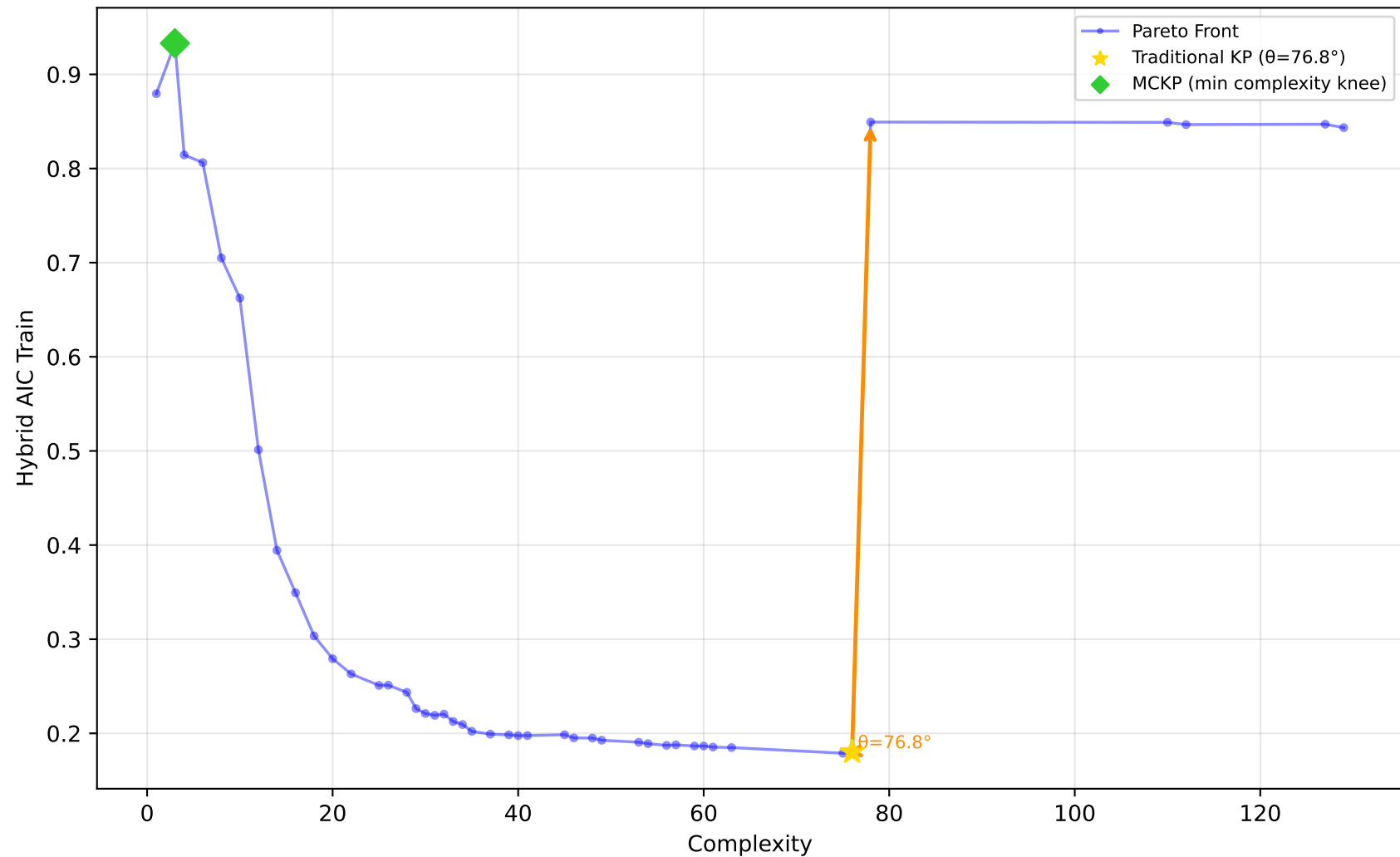
227_cpu_small - Run 27 - MVP - Hybrid AIC Train \lambda_1=0.80, \bar{\lambda}_2=0.20, \lambda_3=0.00 | Difficulty: 1.00 | Method: hmr
