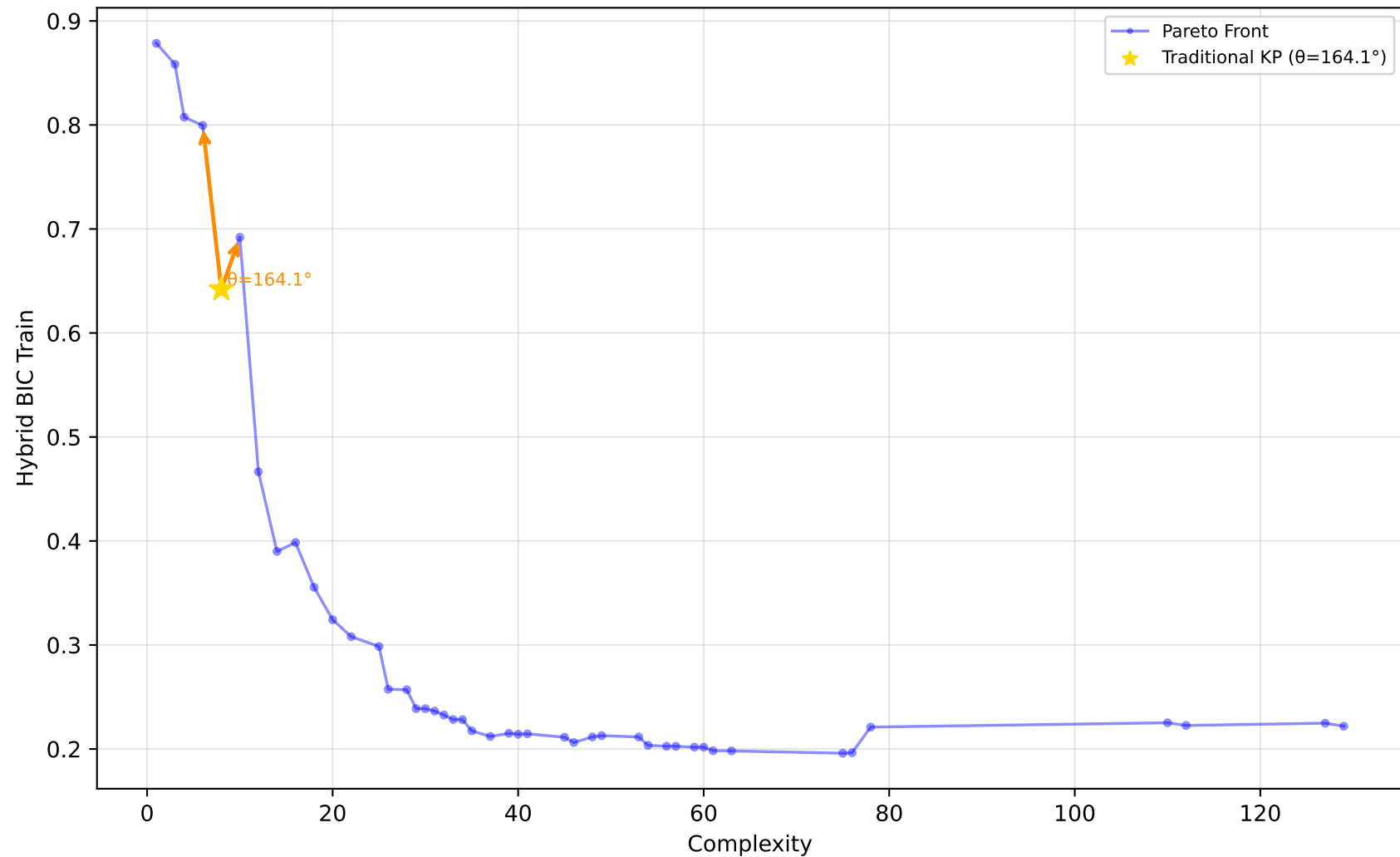
227_cpu_small - Run 27 - MVP - Hybrid BIC Train \lambda_1=0.00, \lambda_2=0.90, \lambda_3=0.10 | Difficulty: 1.00 | Method: hmr
