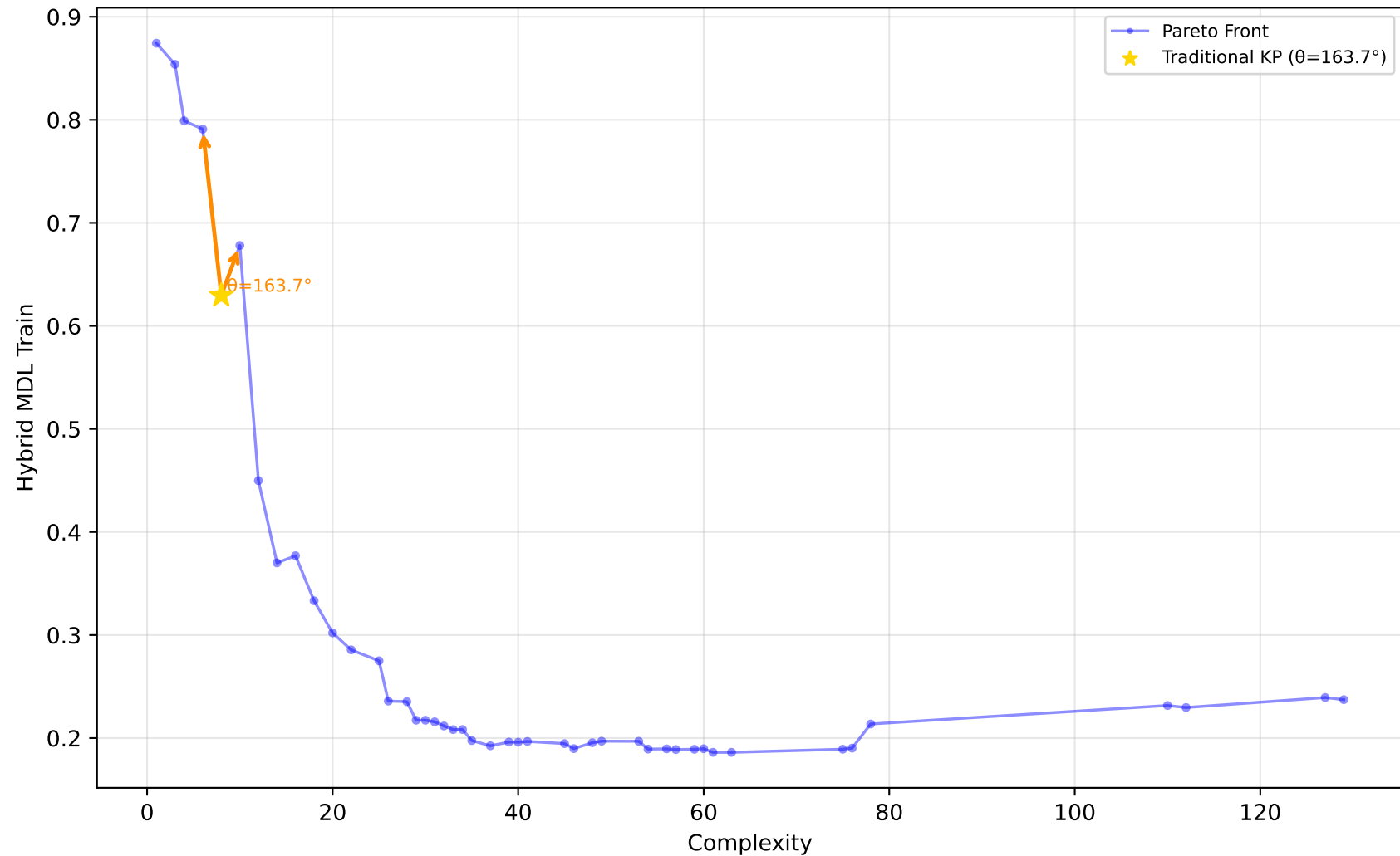
227_cpu_small - Run 27 - MVP - Hybrid MDL Train \lambda_1=0.00, \lambda_2=0.90, \lambda_3=0.10 | Difficulty: 1.00 | Method: hmr
