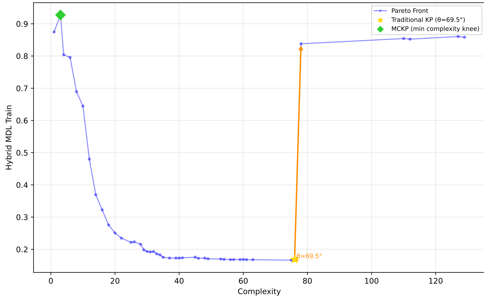
227_cpu_small - Run 27 - MVP - Hybrid MDL Train \lambda_1=0.80, \lambda_2=0.20, \lambda_3=0.00 | Difficulty: 1.00 | Method: hmr
