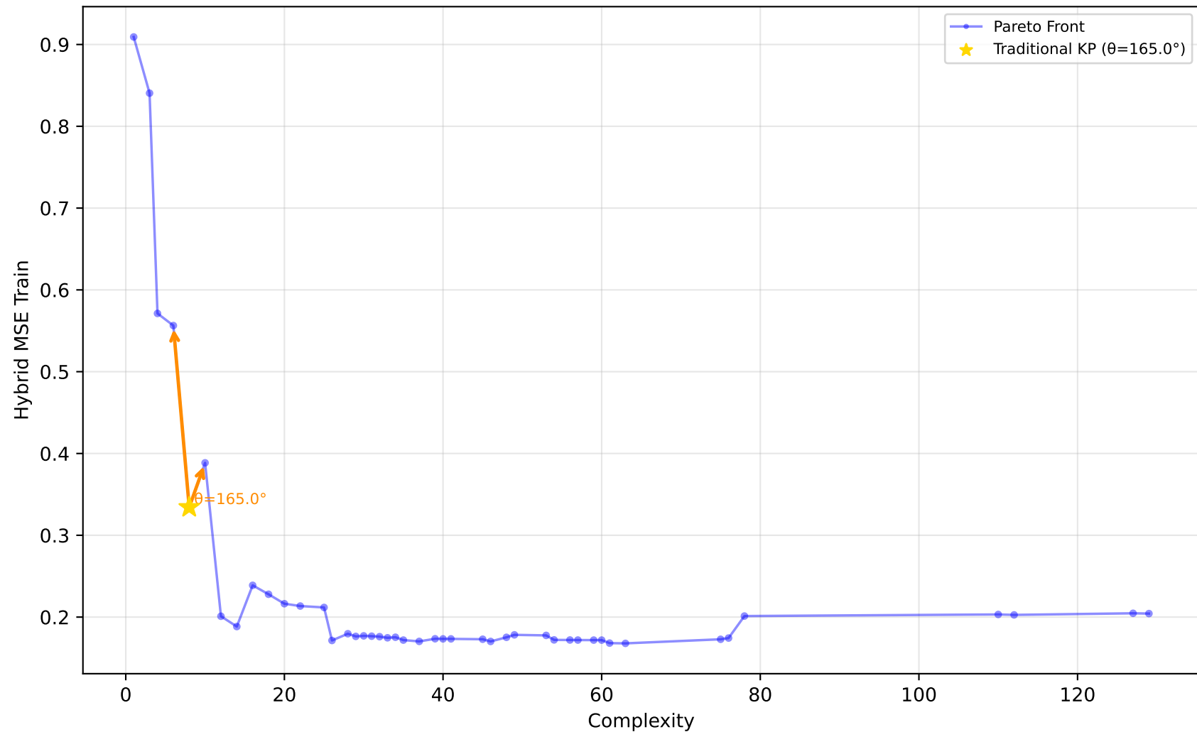
227_cpu_small - Run 27 - MVP - Hybrid MSE Train \lambda_1=0.00, \lambda_2=0.90, \lambda_3=0.10 | Difficulty: 1.00 | Method: hmr
