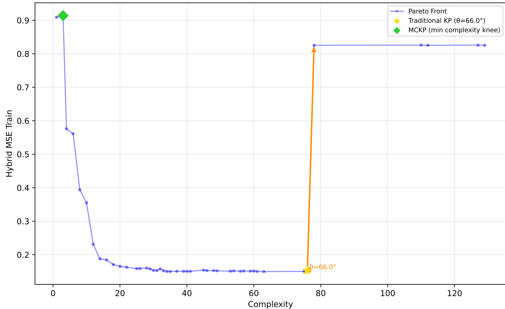
227_cpu_small - Run 27 - MVP - Hybrid MSE Train \lambda_1=0.80, \lambda_2=0.20, \lambda_3=0.00 | Difficulty: 1.00 | Method: hmr
