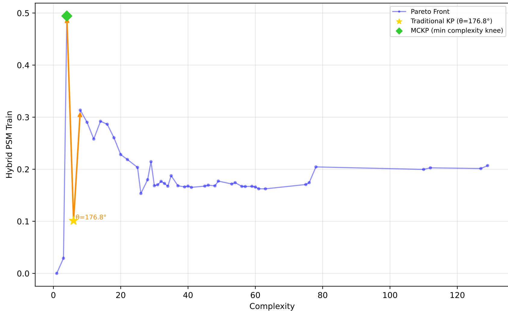
227_cpu_small - Run 27 - MVP - Hybrid PSM Train \lambda_1=0.00, \lambda_2=0.90, \lambda_3=0.10 | Difficulty: 1.00 | Method: hmr
