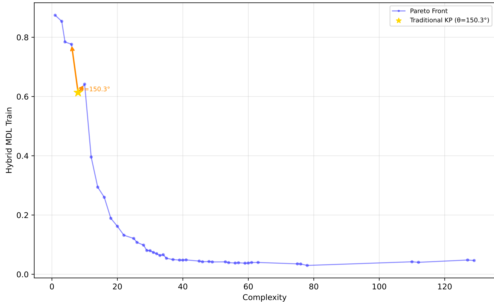
227_cpu_small - Run 27 - SVP - Hybrid MDL Train \lambda_1=0.00, \lambda_2=1.00, \lambda_3=0.00 | Difficulty: 1.00 | Method: hmr
