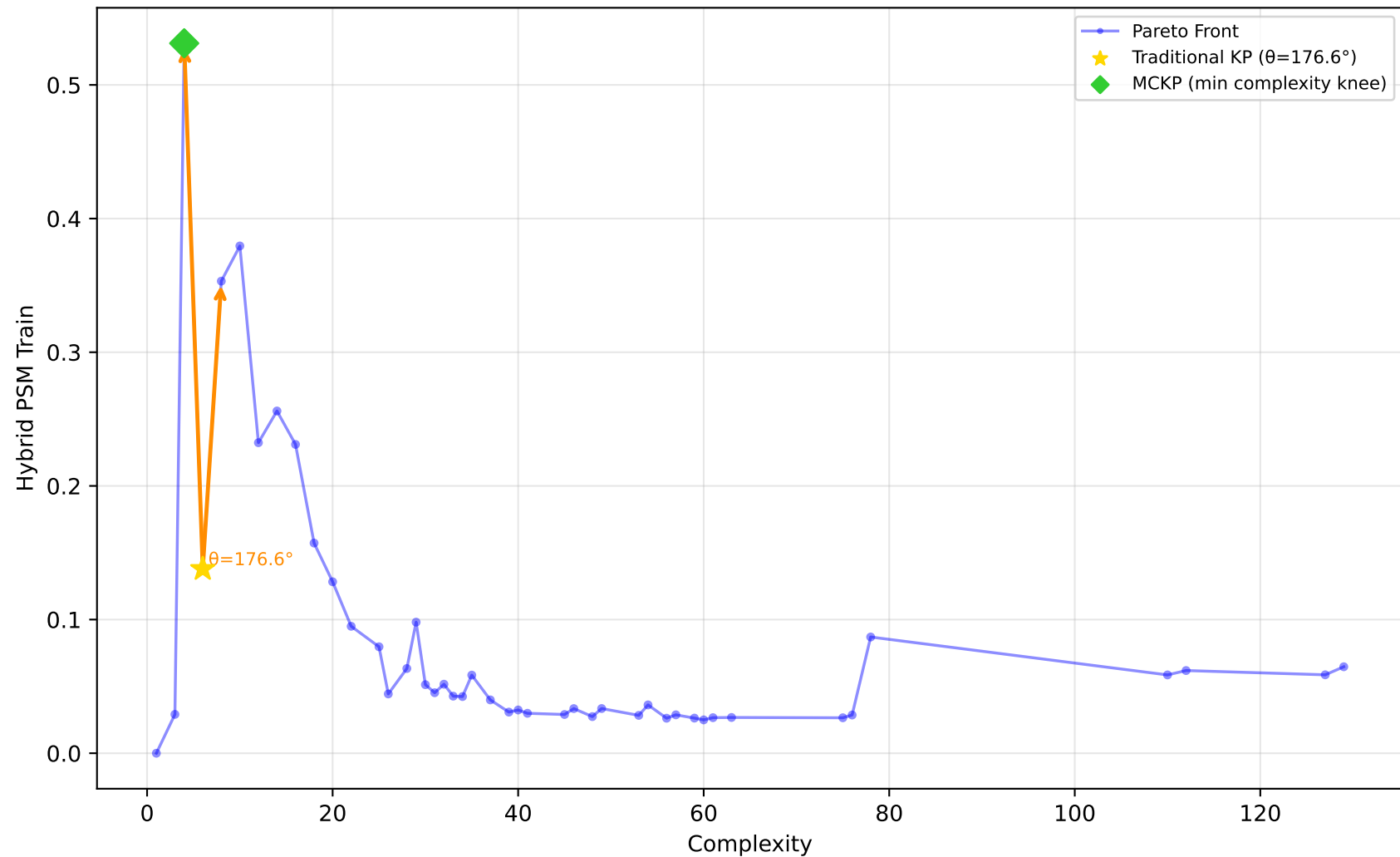
227_cpu_small - Run 27 - SVP - Hybrid PSM Train \lambda_1=0.00, \lambda_2=0.80, \lambda_3=0.30 | Difficulty: 1.00 | Method: hmr
