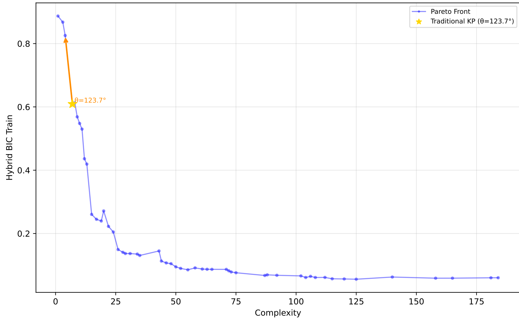
227_cpu_small - Run 28 - MVP - Hybrid BIC Train \lambda_1=0.00, \lambda_2=0.90, \lambda_3=0.10 | Difficulty: 1.00 | Method: hmr
