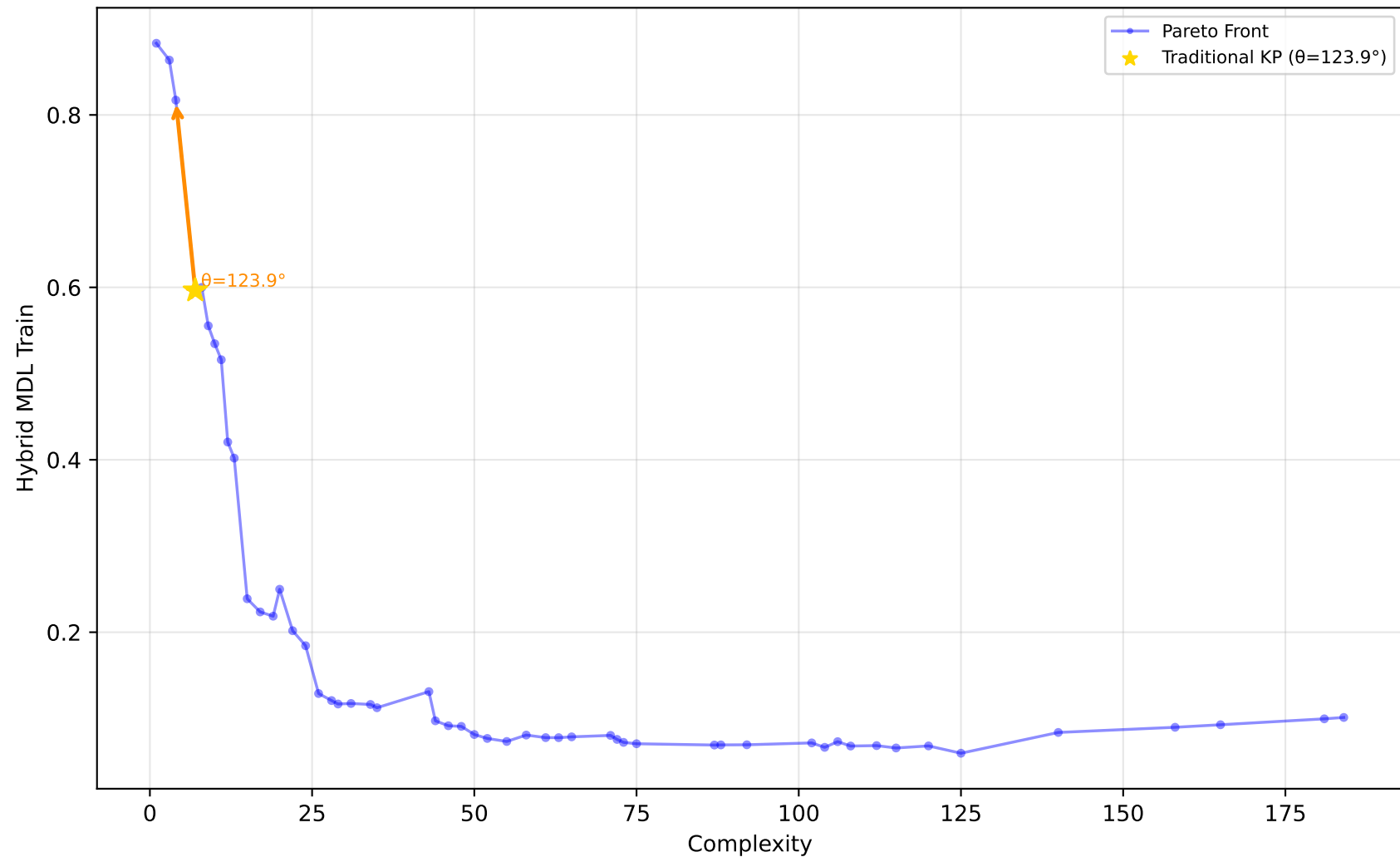
227_cpu_small - Run 28 - MVP - Hybrid MDL Train \lambda_1=0.00, \lambda_2=0.90, \lambda_3=0.10 | Difficulty: 1.00 | Method: hmr
