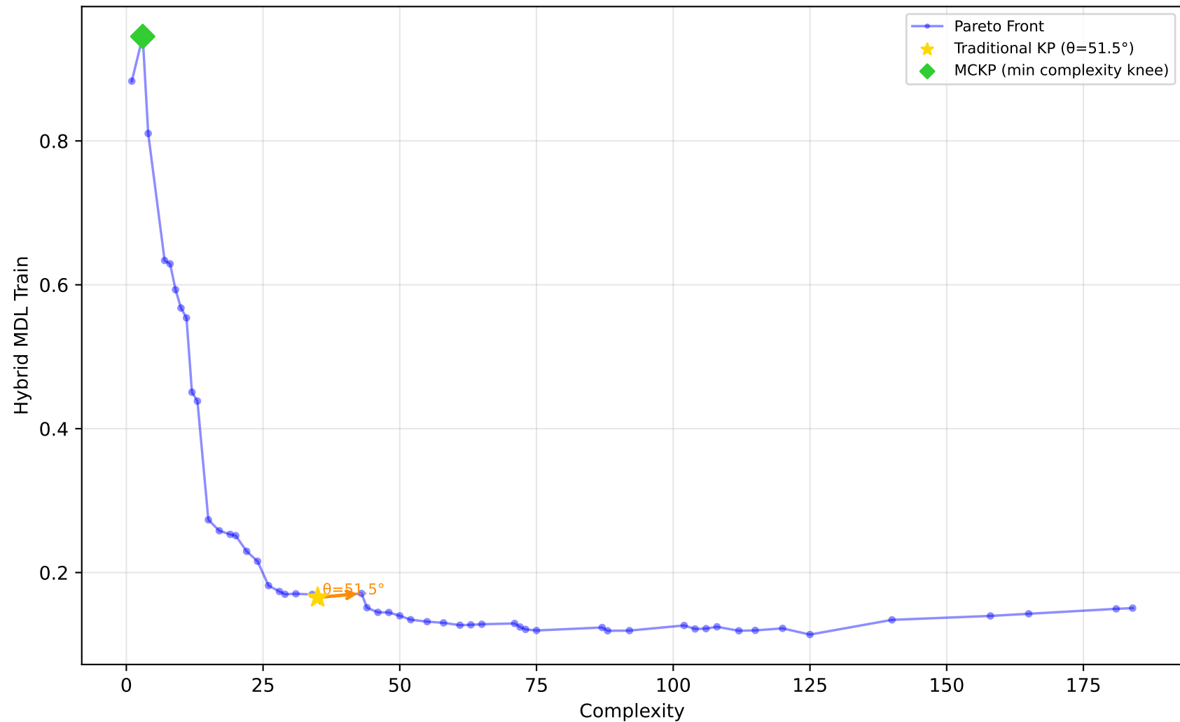
227_cpu_small - Run 28 - MVP - Hybrid MDL Train \lambda_1=0.80, \lambda_2=0.20, \lambda_3=0.00 | Difficulty: 1.00 | Method: hmr
