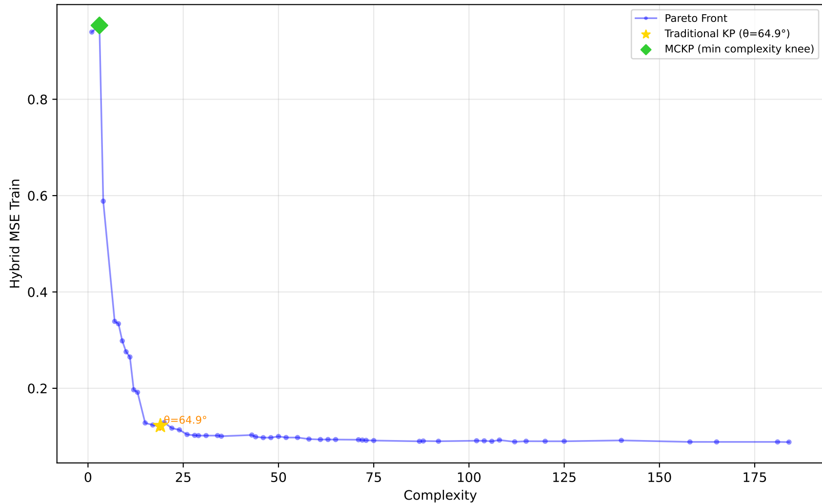
227_cpu_small - Run 28 - MVP - Hybrid MSE Train \lambda_1=0.80, \lambda_2=0.20, \lambda_3=0.00 | Difficulty: 1.00 | Method: hmr
