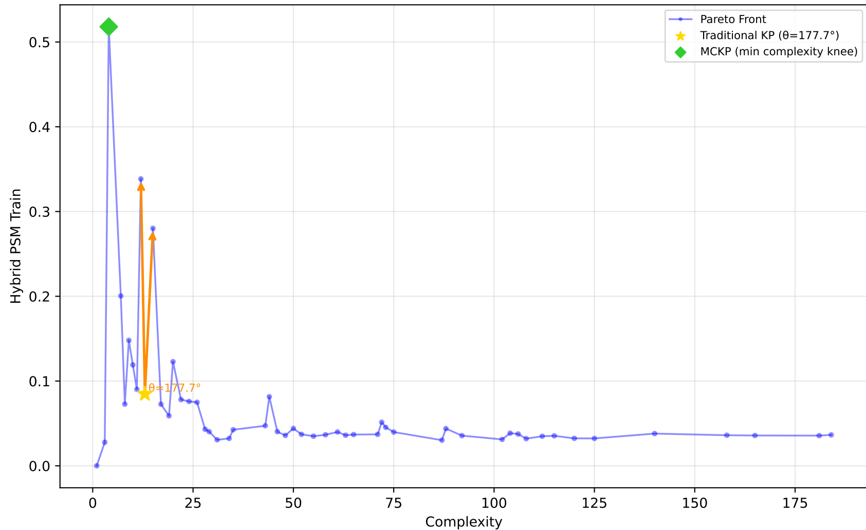
227_cpu_small - Run 28 - MVP - Hybrid PSM Train \lambda_1=0.00, \lambda_2=0.90, \lambda_3=0.10 | Difficulty: 1.00 | Method: hmr
