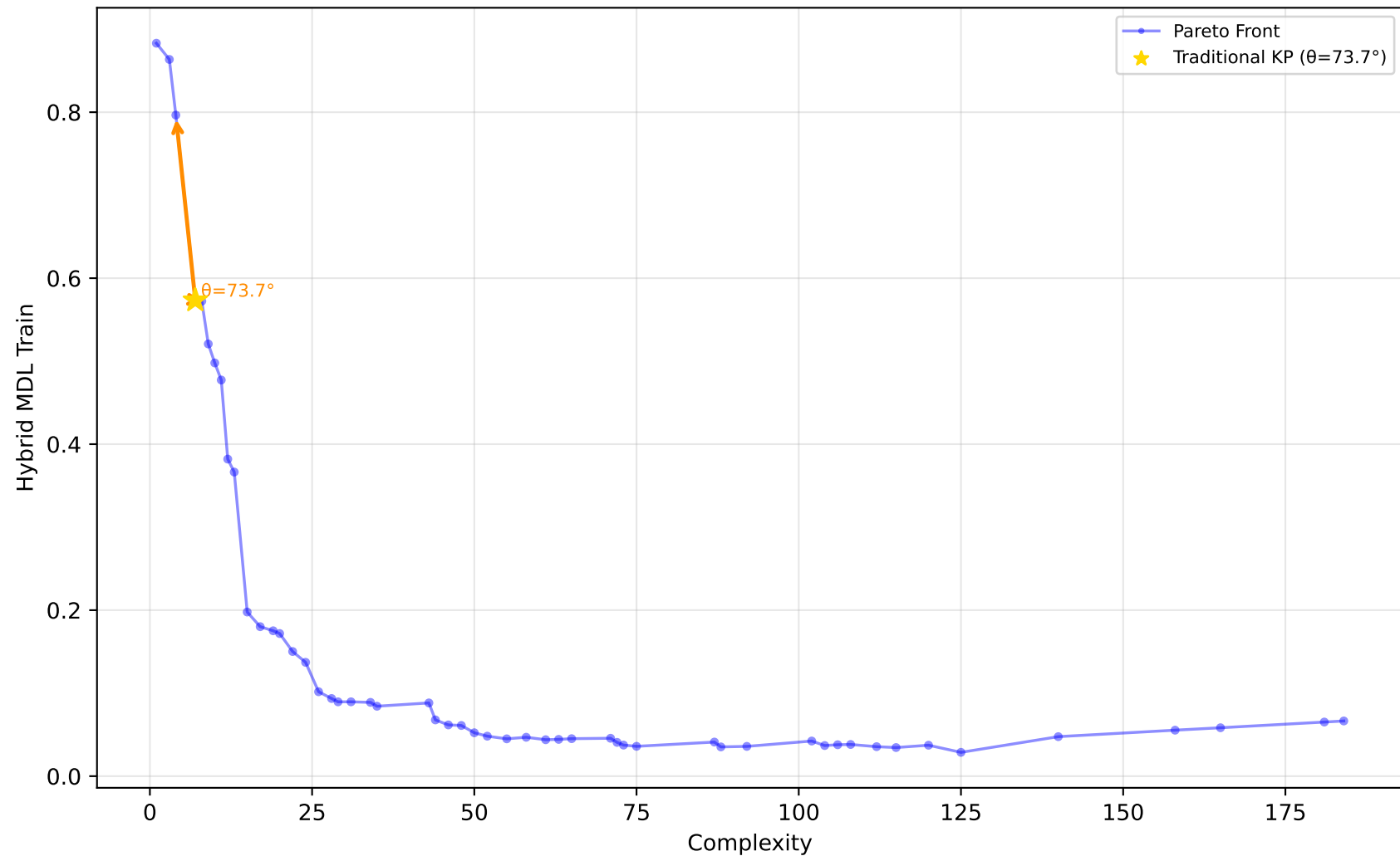
227_cpu_small - Run 28 - SVP - Hybrid MDL Train \lambda_1=0.00, \lambda_2=1.00, \lambda_3=0.00 | Difficulty: 1.00 | Method: hmr
