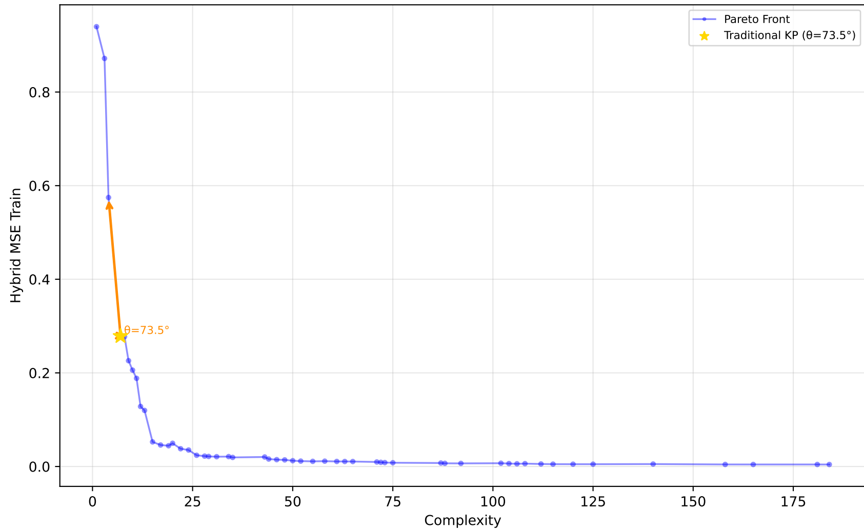
227_cpu_small - Run 28 - SVP - Hybrid MSE Train \lambda_1=0.00, \lambda_2=1.00, \lambda_3=0.00 | Difficulty: 1.00 | Method: hmr
