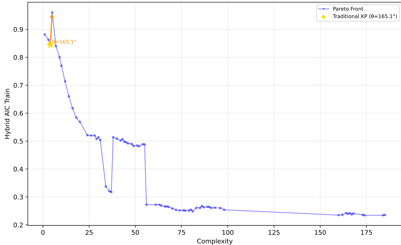
227_cpu_small - Run 29 - MVP - Hybrid AIC Train \lambda_1=0.00, \bar{\lambda}_2=0.90, \lambda_3=0.10 | Difficulty: 1.00 | Method: hmr
