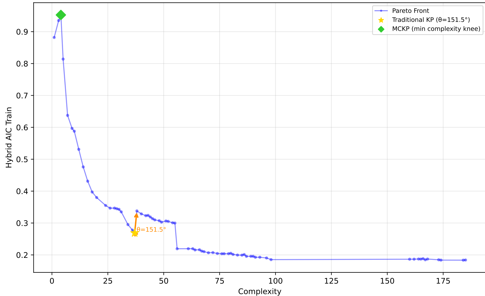
227_cpu_small - Run 29 - MVP - Hybrid AIC Train \lambda_1=0.80, \lambda_2=0.20, \lambda_3=0.00 | Difficulty: 1.00 | Method: hmr
