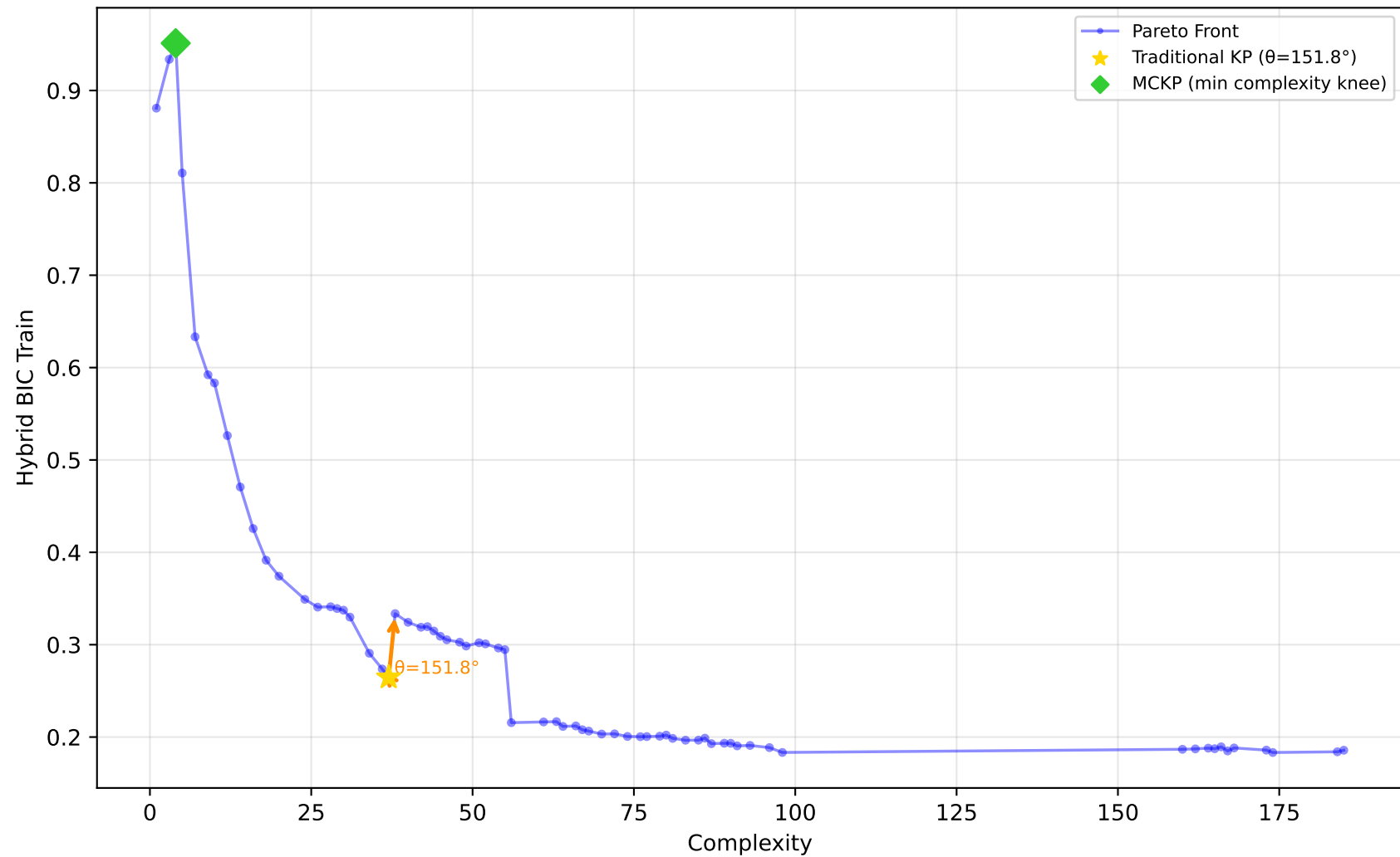
227_cpu_small - Run 29 - MVP - Hybrid BIC Train \lambda_1=0.80, \bar{\lambda}_2=0.20, \lambda_3=0.00 | Difficulty: 1.00 | Method: hmr
