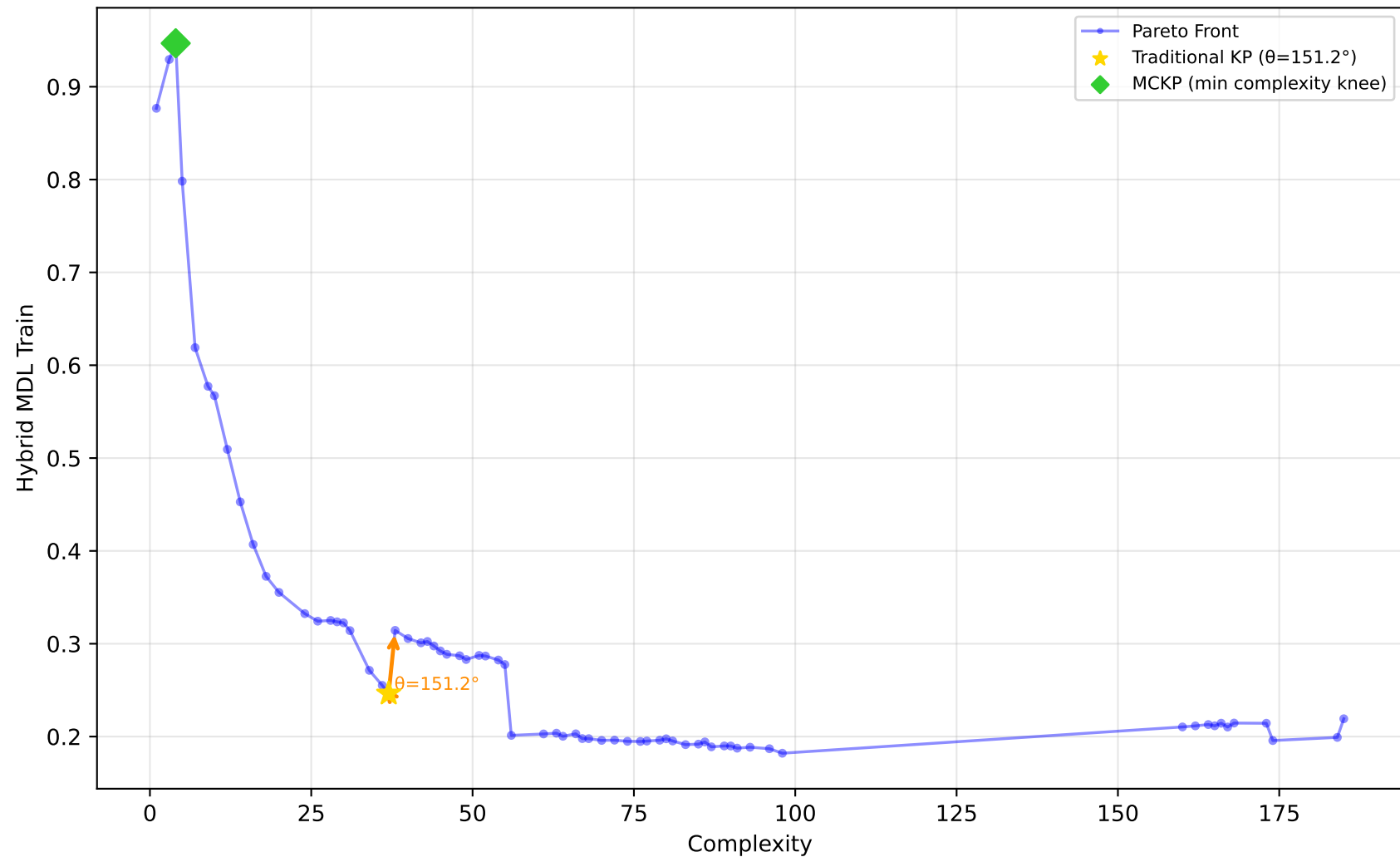
227_cpu_small - Run 29 - MVP - Hybrid MDL Train \lambda_1=0.80, \lambda_2=0.20, \lambda_3=0.00 | Difficulty: 1.00 | Method: hmr
