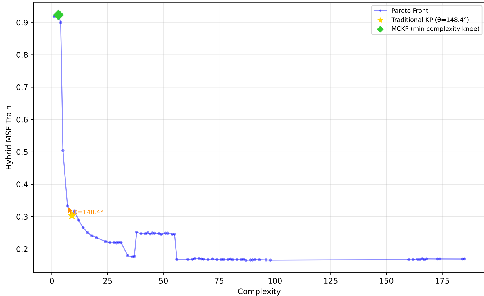
227_cpu_small - Run 29 - MVP - Hybrid MSE Train \lambda_1=0.80, \lambda_2=0.20, \lambda_3=0.00 | Difficulty: 1.00 | Method: hmr
