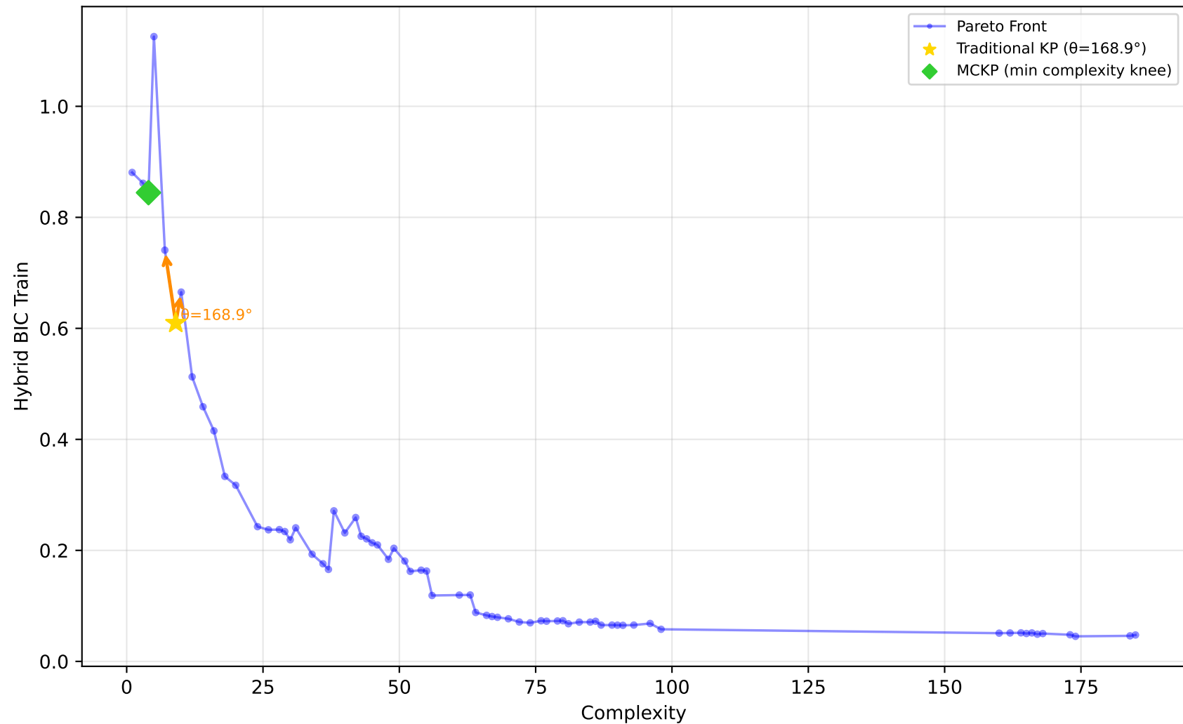
227_cpu_small - Run 29 - SVP - Hybrid BIC Train \lambda_1=0.00, \bar{\lambda}_2=0.80, \lambda_3=0.30 | Difficulty: 1.00 | Method: hmr
