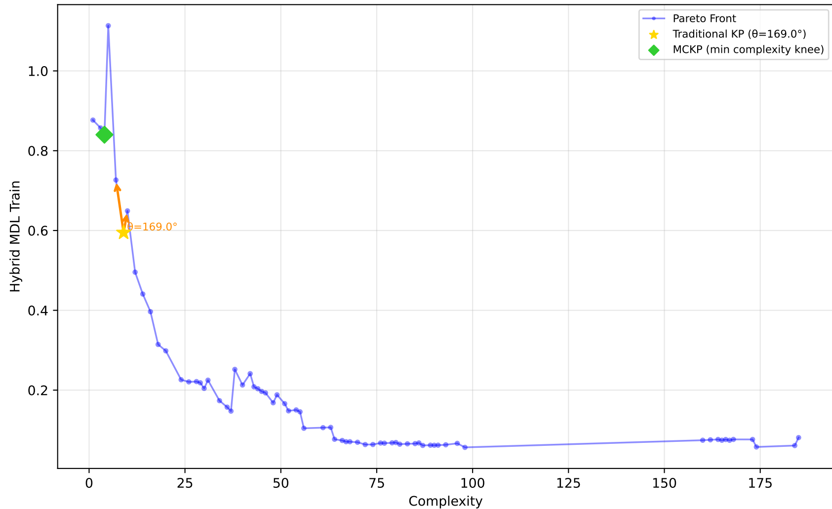
227_cpu_small - Run 29 - SVP - Hybrid MDL Train \lambda_1=0.00, \lambda_2=0.80, \lambda_3=0.30 | Difficulty: 1.00 | Method: hmr
