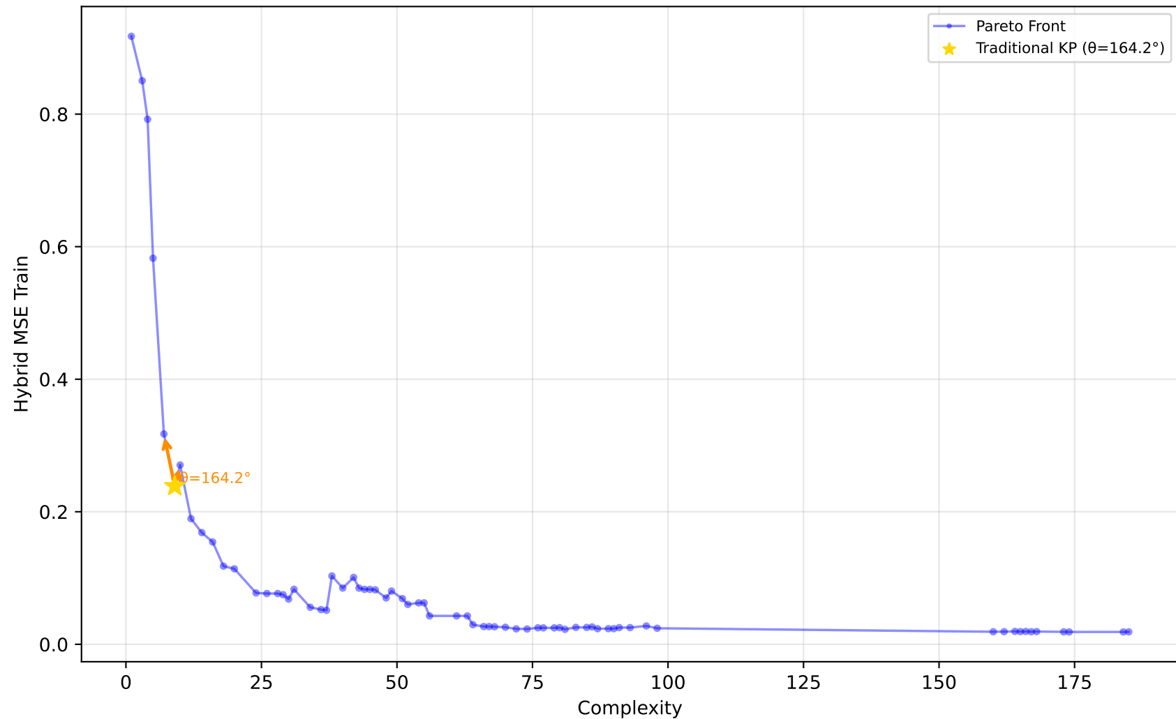
227_cpu_small - Run 29 - SVP - Hybrid MSE Train \lambda_1=0.00, \lambda_2=1.00, \lambda_3=0.00 | Difficulty: 1.00 | Method: hmr
