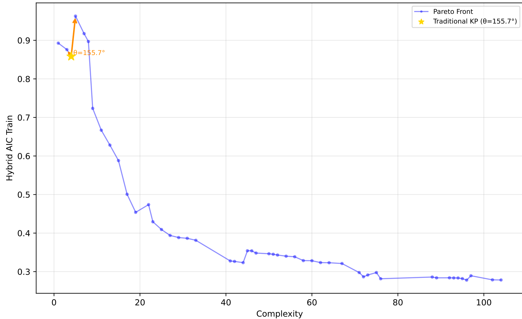
227_cpu_small - Run 2 - MVP - Hybrid AIC Train \lambda_1=0.00, \bar{\lambda}_2=0.90, \lambda_3=0.10 | Difficulty: 1.00 | Method: hmr
