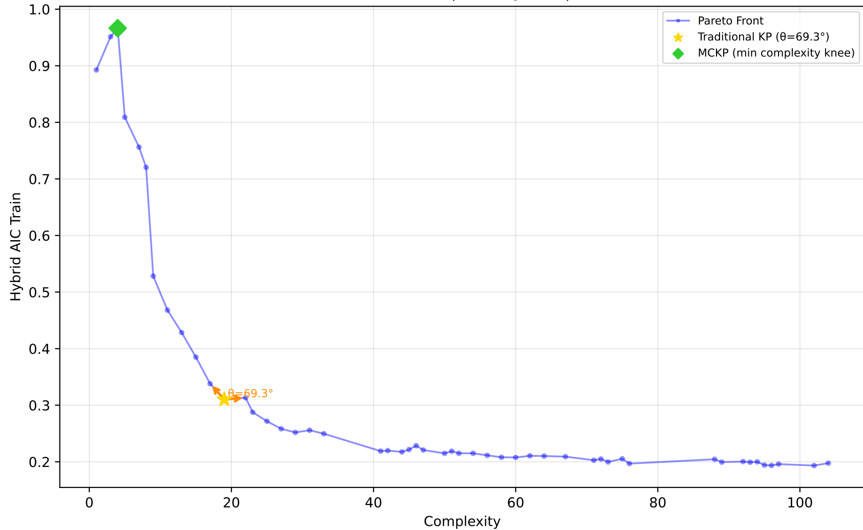
227_cpu_small - Run 2 - MVP - Hybrid AIC Train \lambda_1=0.80, \bar{\lambda}_2=0.20, \lambda_3=0.00 | Difficulty: 1.00 | Method: hmr
