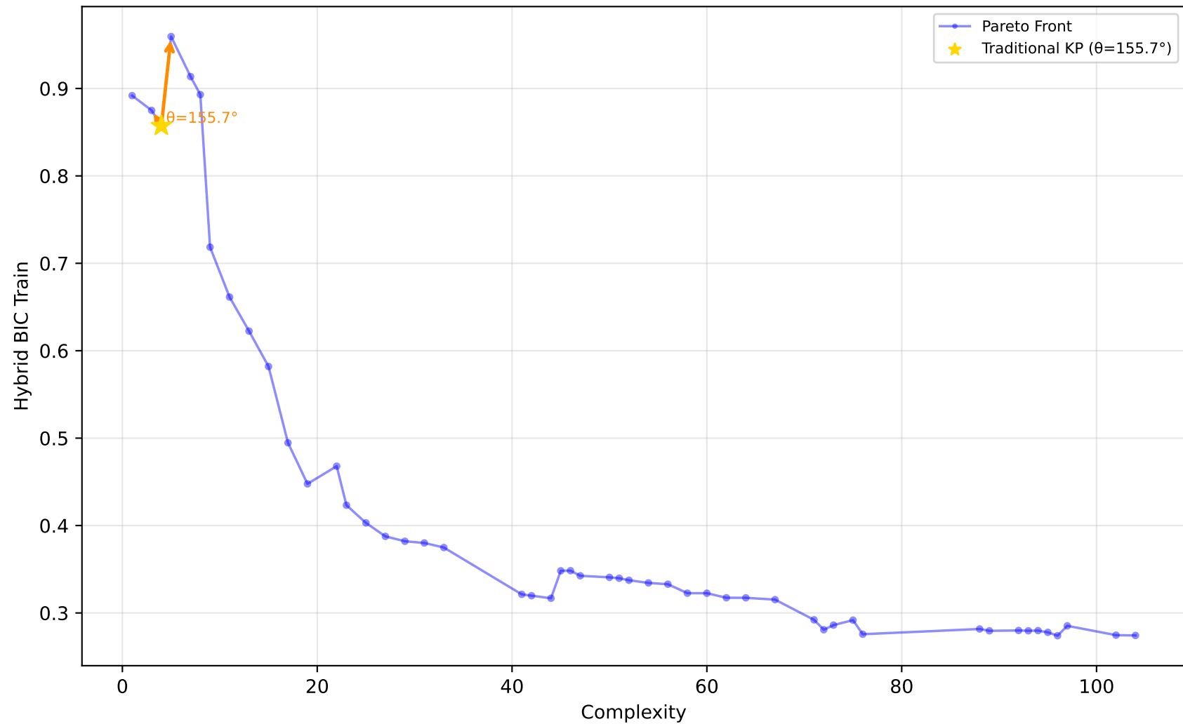
227_cpu_small - Run 2 - MVP - Hybrid BIC Train \lambda_1=0.00, \bar{\lambda}_2=0.90, \lambda_3=0.10 | Difficulty: 1.00 | Method: hmr
