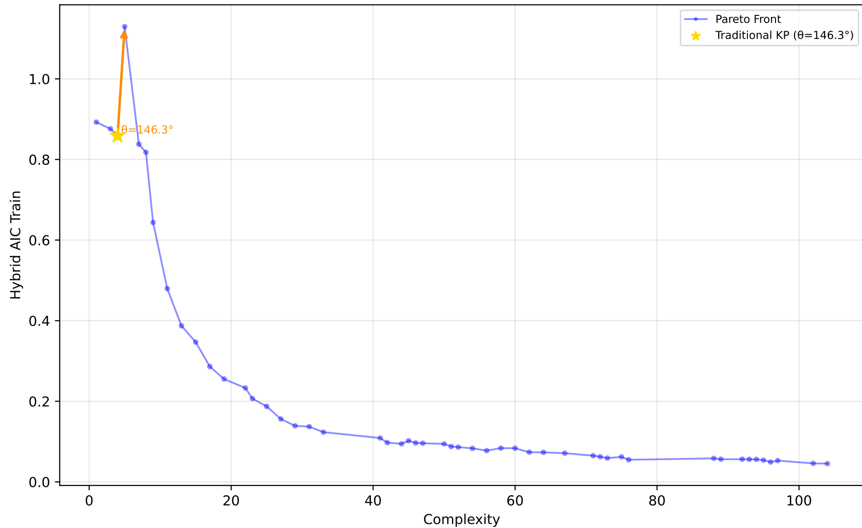
227_cpu_small - Run 2 - SVP - Hybrid AIC Train \lambda_1=0.00, \bar{\lambda}_2=0.80, \lambda_3=0.30 | Difficulty: 1.00 | Method: hmr
