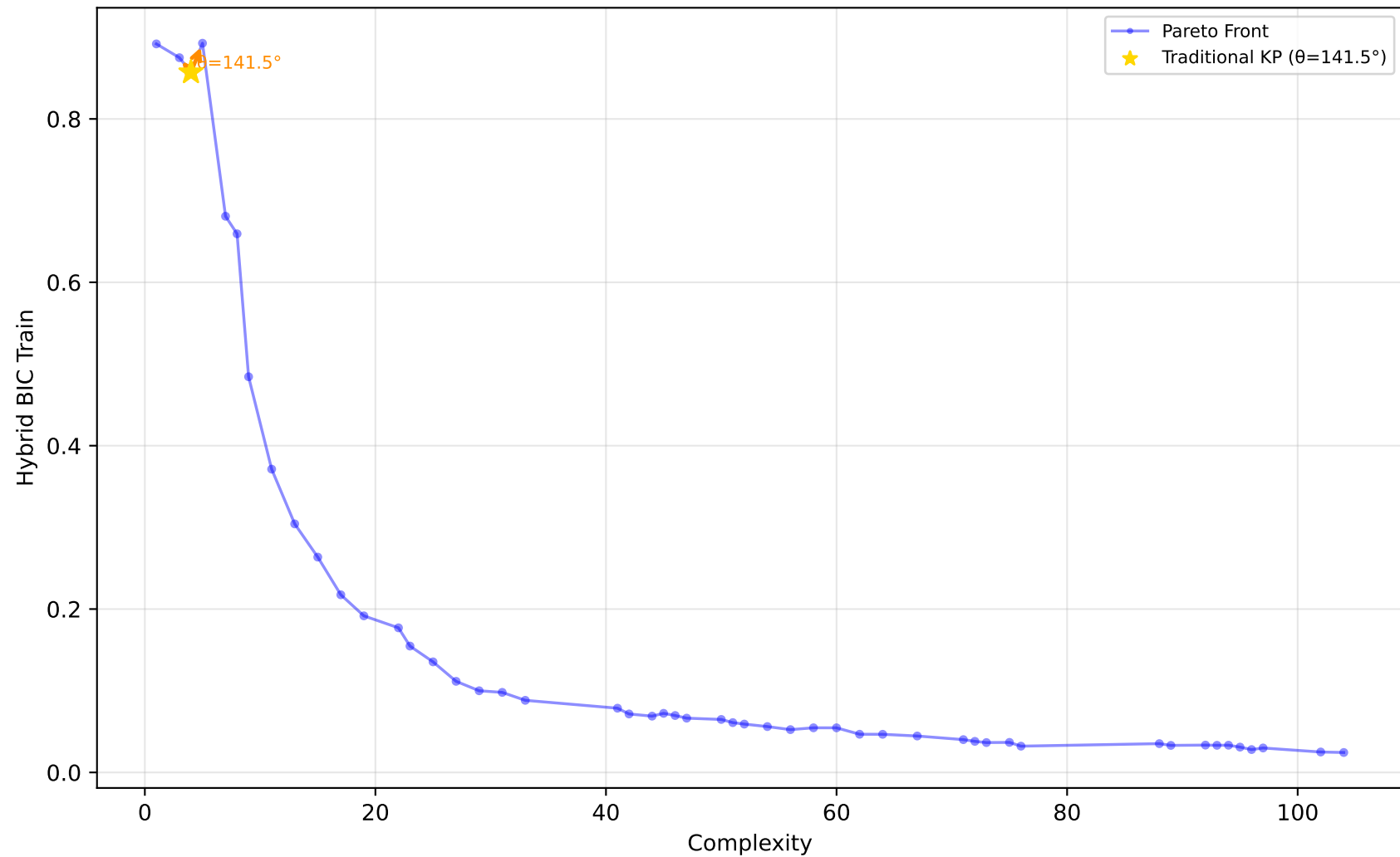
227_cpu_small - Run 2 - SVP - Hybrid BIC Train \lambda_1=0.00, \lambda_2=1.00, \lambda_3=0.00 | Difficulty: 1.00 | Method: hmr
