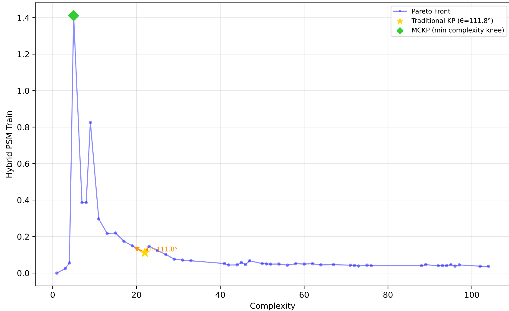
227_cpu_small - Run 2 - SVP - Hybrid PSM Train \lambda_1=0.00, \lambda_2=0.80, \lambda_3=0.30 | Difficulty: 1.00 | Method: hmr
